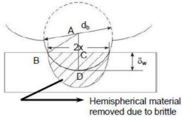
Interaction between grit and workpiece and tool
