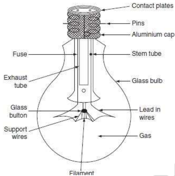
(Fig.4.3. Construction of Filament Lamp)
