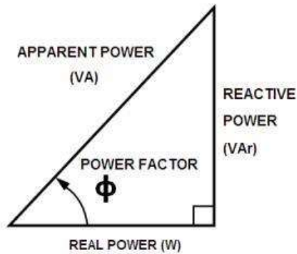
(Fig.2.20.Power Triangle)
