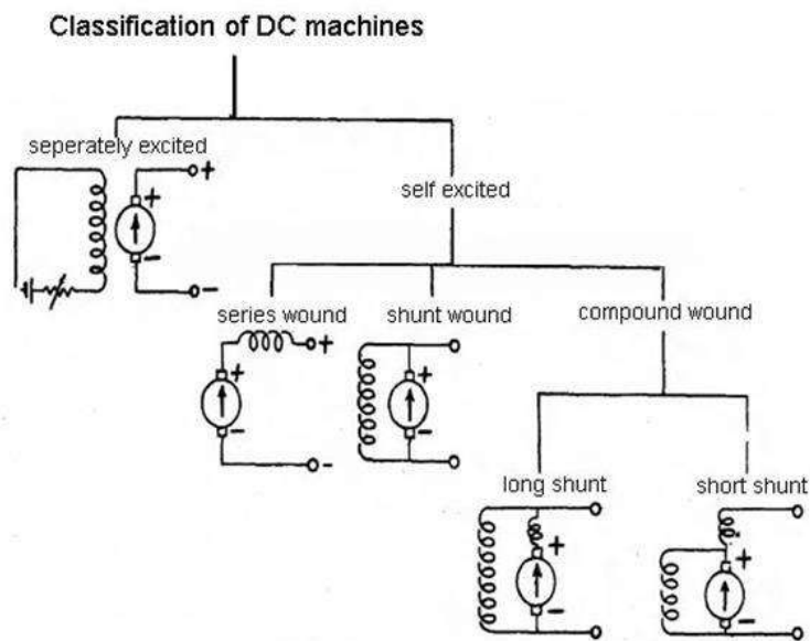
(Fig.4.2. Classification of DC machine)
