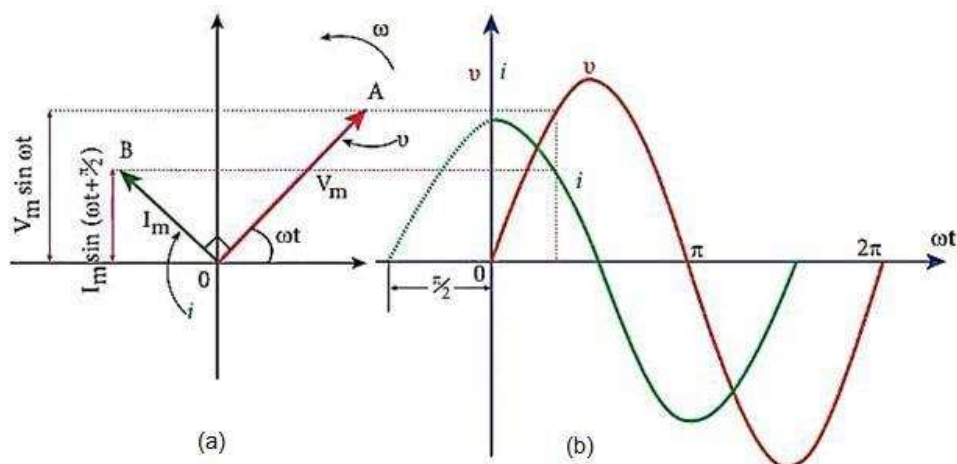
(Fig.2.14.(a) Phasor representation of voltage and current in pure capacitive circuit (b) Wave representation of voltage and current in pure capacitive circuit)
