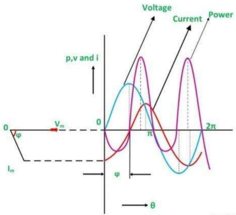
(Fig.2.16. waveform representation of R-L circuit)
