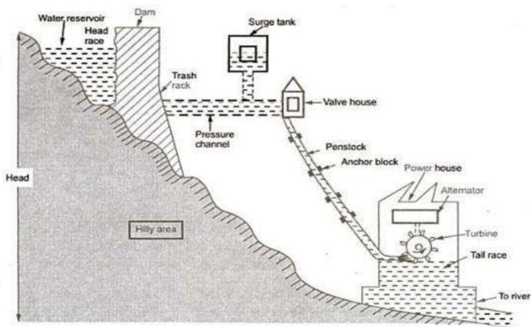
(Fig.3.2. Block Diagram of Hydro Power Plant)
